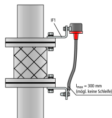
Installation of EXFS L200
