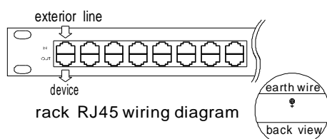
LDY-RJ45/L wiring diagram
